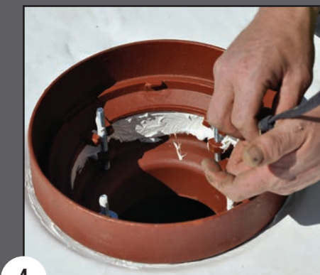
4 Seal free edges of membrane with urethane sealant.
